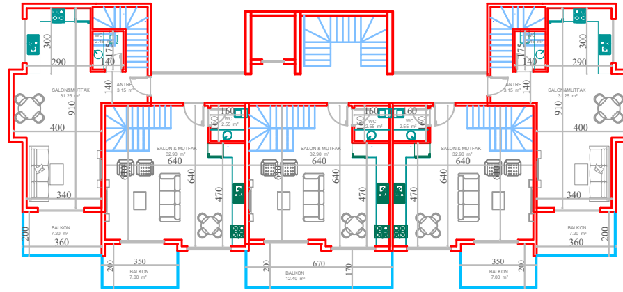
2. KAT PLANI
