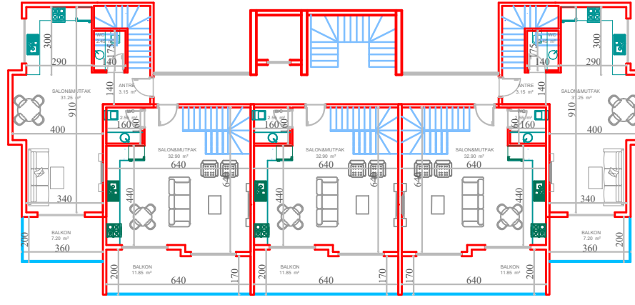
BODRUM KAT PLANI
