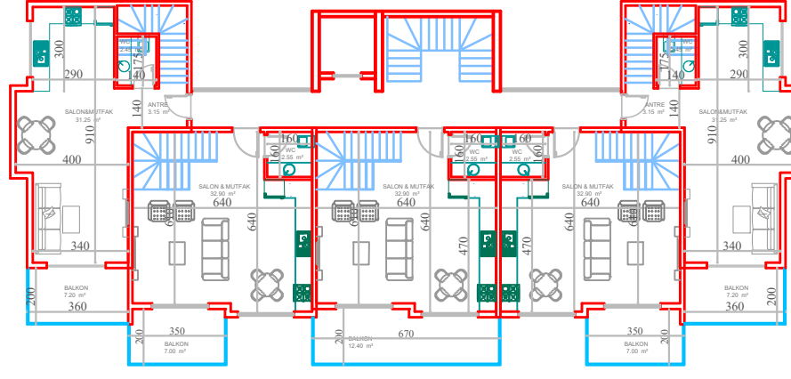
2. KAT PLANI
